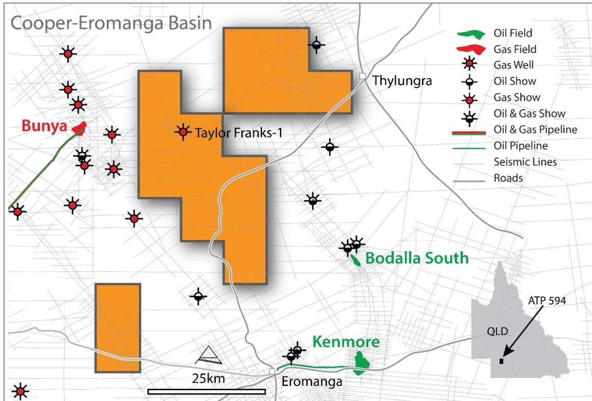
Figure 1: ATP 594 permit and adjacent wells in Cooper-Eromanga Basin
