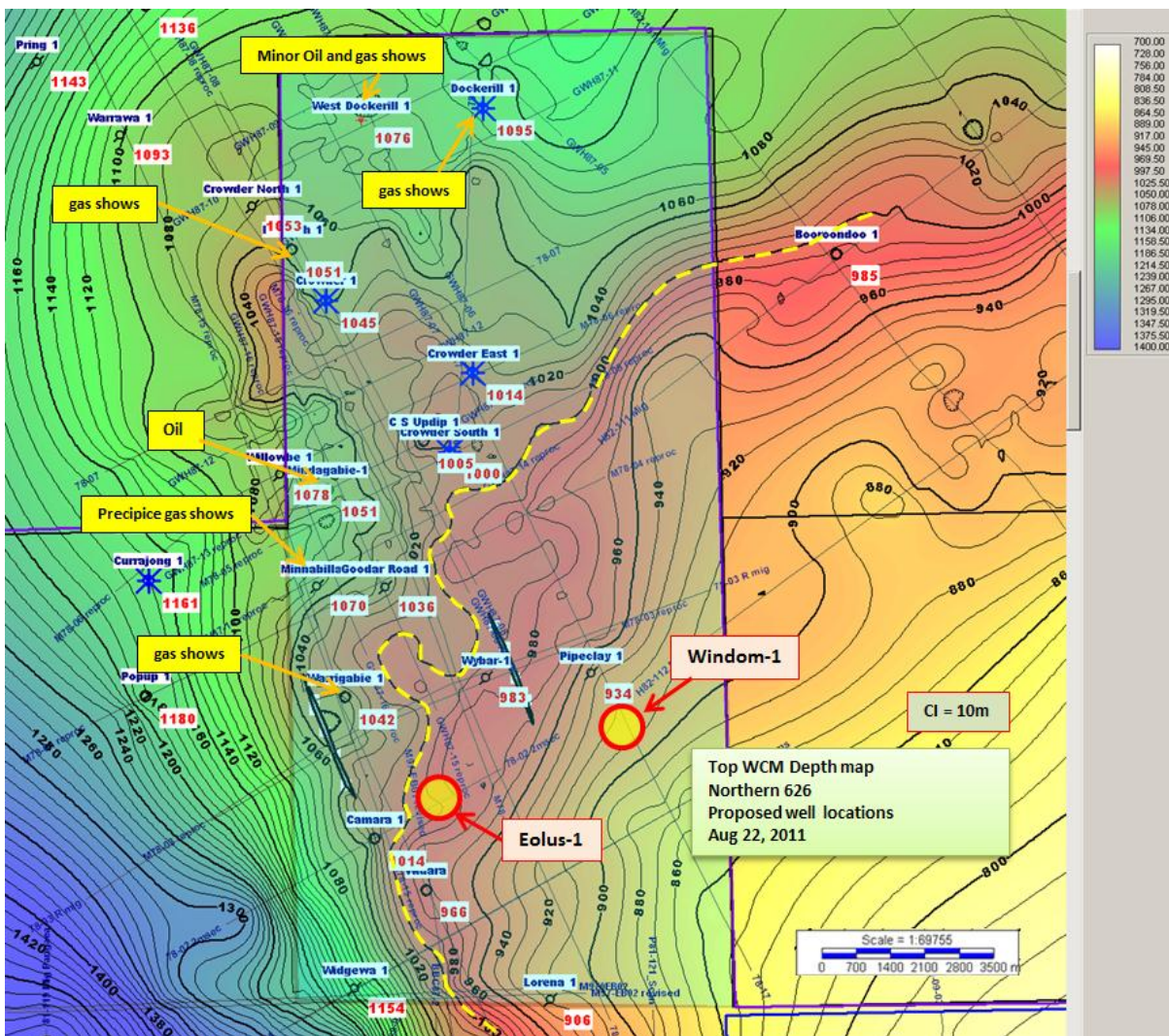
Structure map ATP626P
